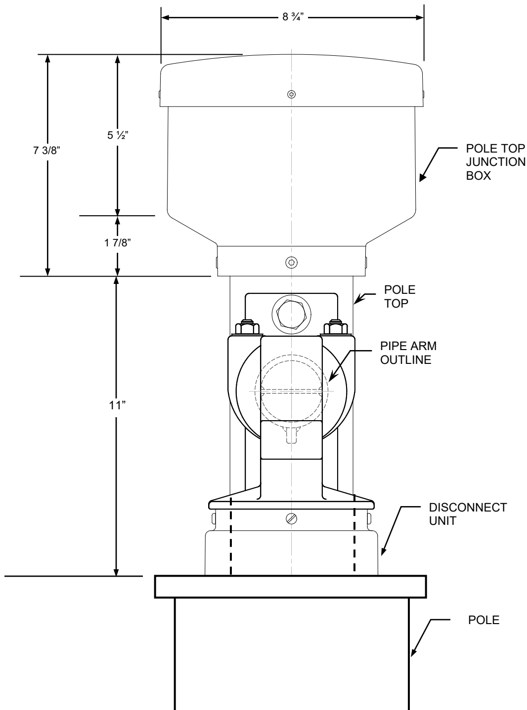
END VIEW
