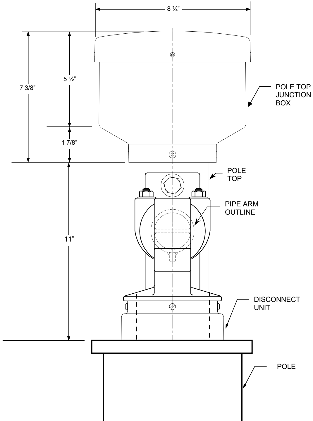
END VIEW
