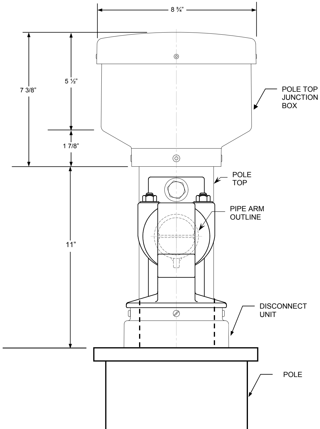
END VIEW
